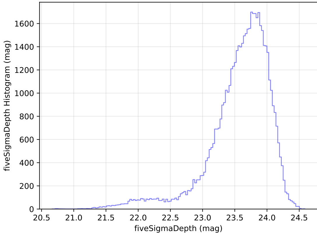
internal_u_expt38_nscale1.5v3.4_10yrs Yr 1 i band: fiveSigmaDepth Histogram
