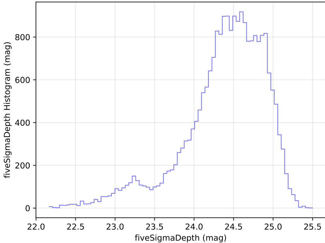
internal_u_expt38_nscale1.5v3.4_10yrs Yr 1 g band: fiveSigmaDepth Histogram
