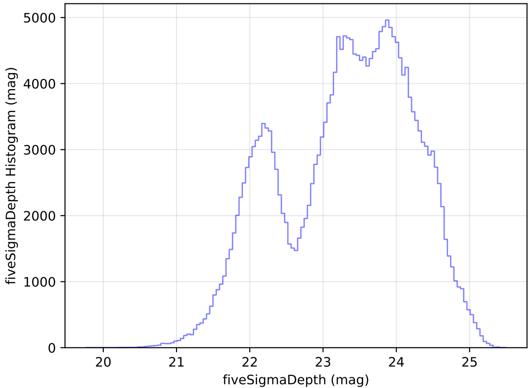
internal_u_expt38_nscale1.5v3.4_10yrs Yr 1 all bands: fiveSigmaDepth Histogram
