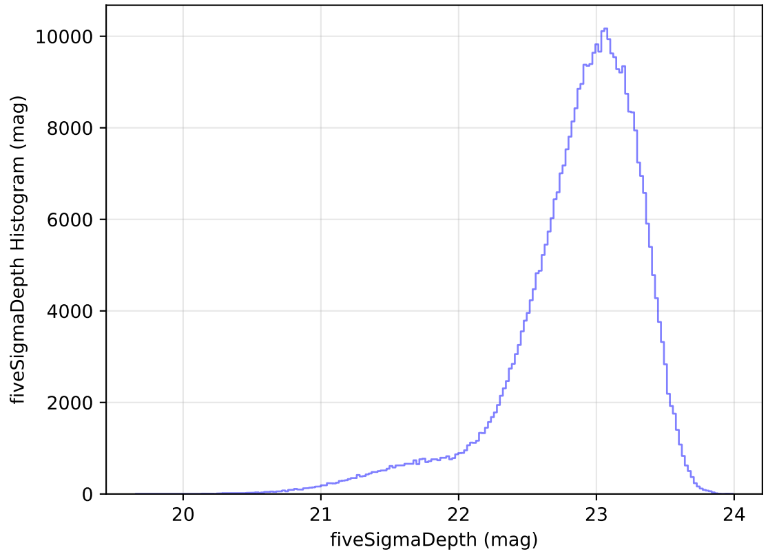
internal_u_expt38_nscale1.5v3.4_10yrs WFD z band: fiveSigmaDepth Histogram
