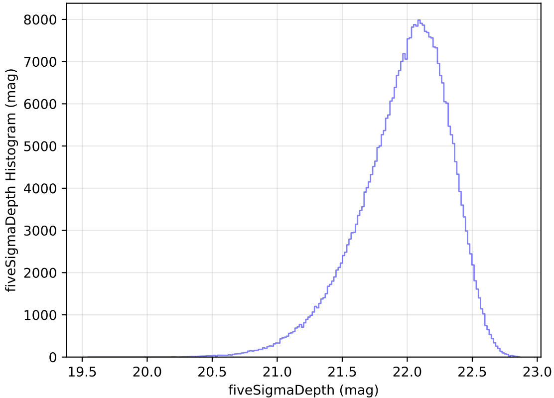
internal_u_expt38_nscale1.5v3.4_10yrs WFD y band: fiveSigmaDepth Histogram
