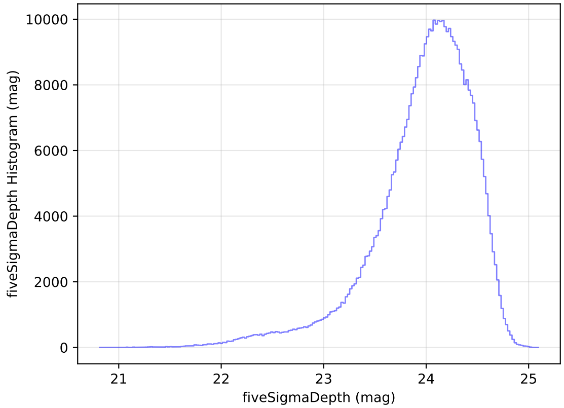
internal_u_expt38_nscale1.5v3.4_10yrs WFD r band: fiveSigmaDepth Histogram
