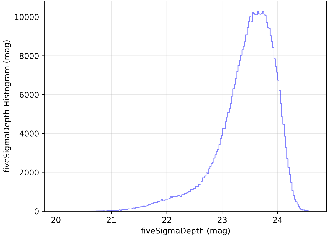
internal_u_expt38_nscale1.5v3.4_10yrs WFD i band: fiveSigmaDepth Histogram
