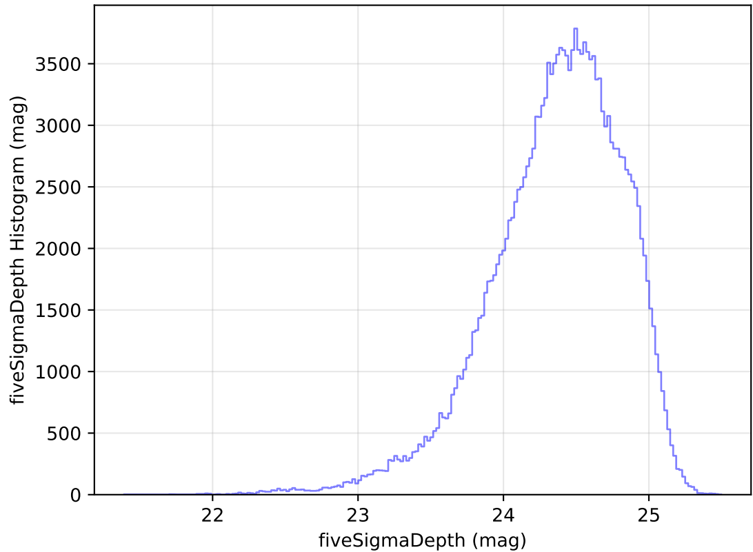
internal_u_expt38_nscale1.5v3.4_10yrs WFD g band: fiveSigmaDepth Histogram
