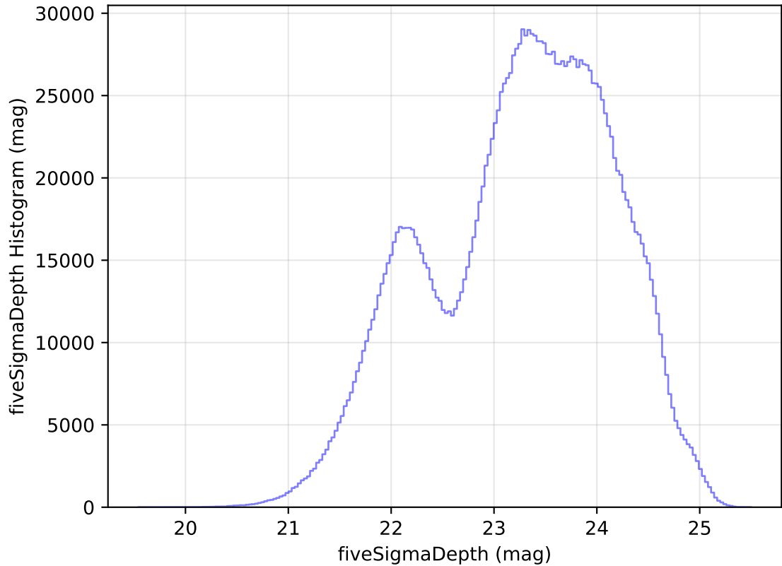
internal_u_expt38_nscale1.5v3.4_10yrs WFD all bands: fiveSigmaDepth Histogram
