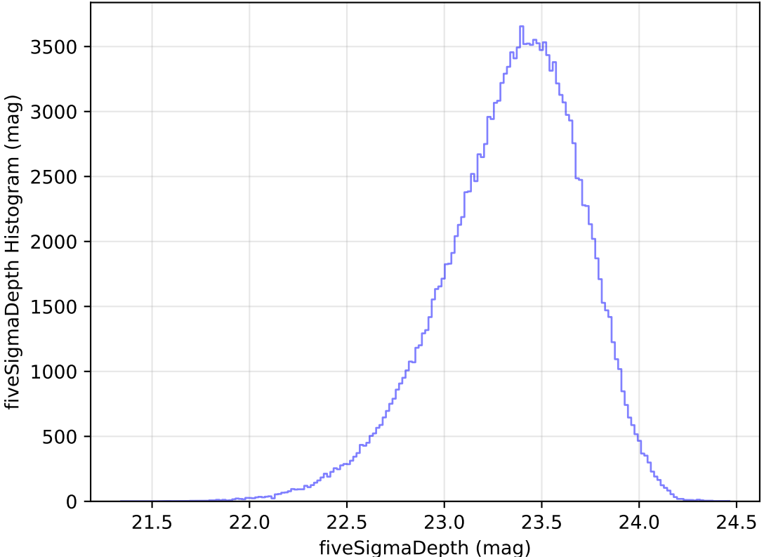
internal_u_expt38_nscale1.5v3.4_10yrs All sky u band: fiveSigmaDepth Histogram
