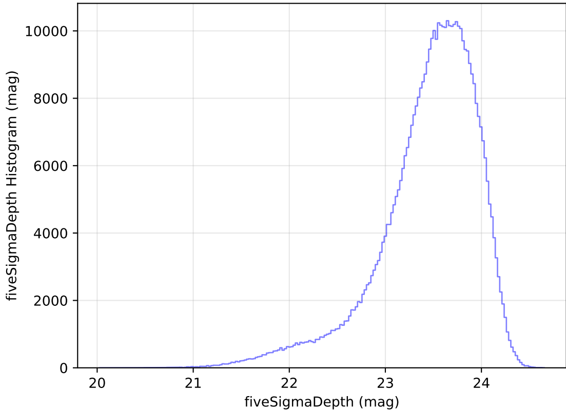
internal_u_expt38_nscale1.5v3.4_10yrs All sky i band: fiveSigmaDepth Histogram
