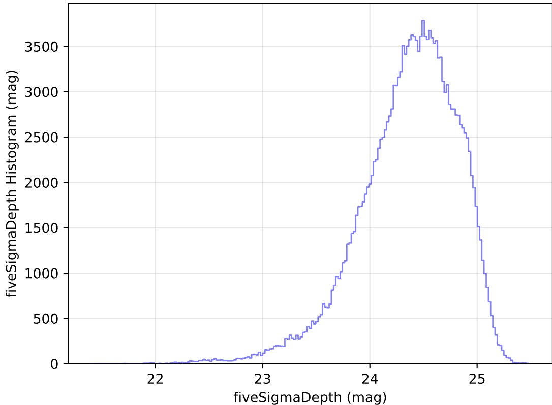
internal_u_expt38_nscale1.5v3.4_10yrs All sky g band: fiveSigmaDepth Histogram
