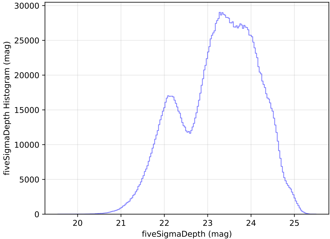
internal_u_expt38_nscale1.5v3.4_10yrs All sky all bands: fiveSigmaDepth Histogram
