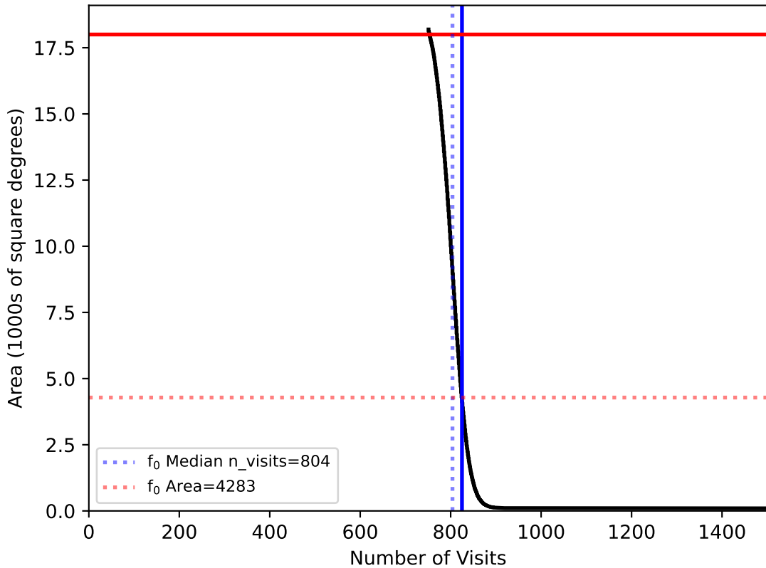
internal_u_expt38_nscale1.5v3.4_10yrs WFD: f0
