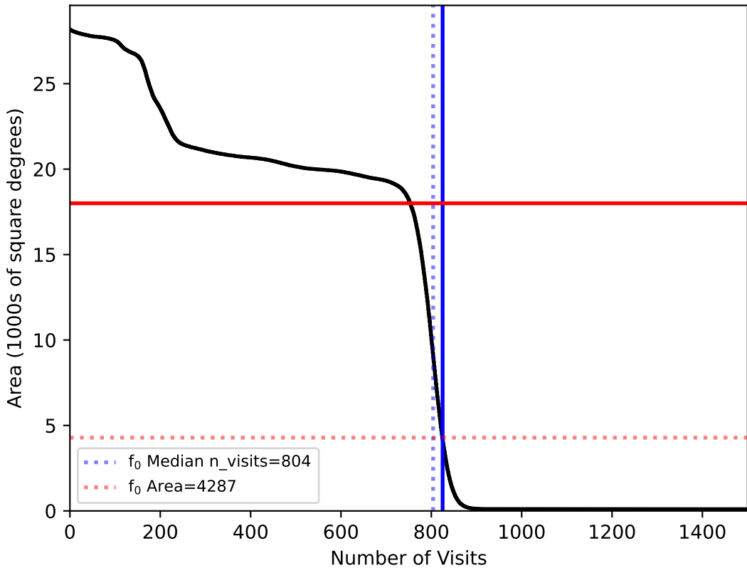
internal_u_expt38_nscale1.5v3.4_10yrs All sky: f0
