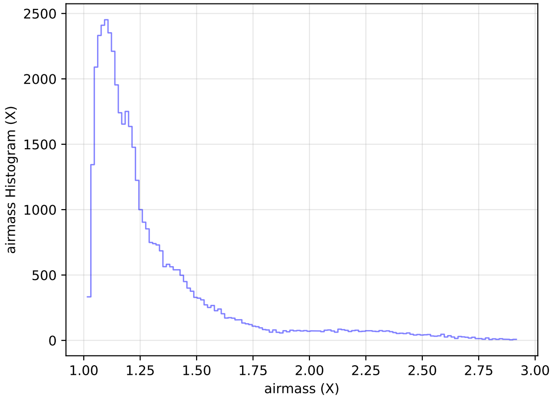
internal_u_expt38_nscale1.5v3.4_10yrs Yr 1 z band: airmass Histogram
