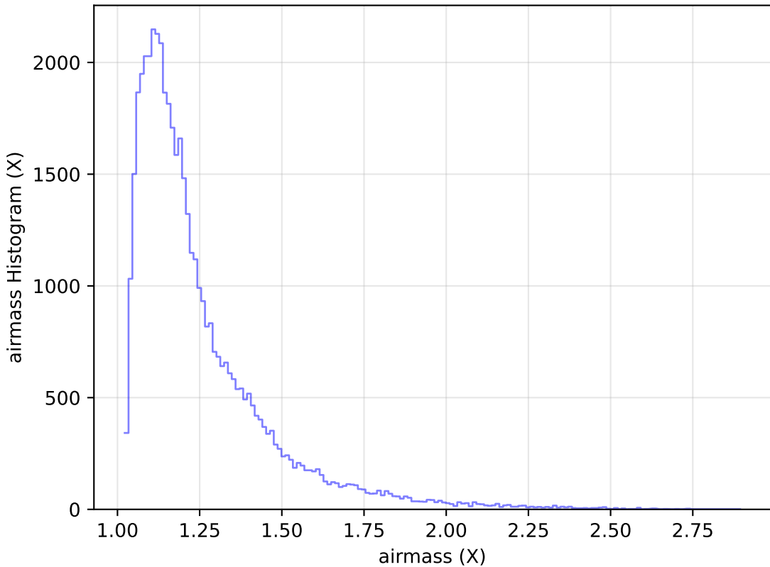
internal_u_expt38_nscale1.5v3.4_10yrs Yr 1 y band: airmass Histogram
