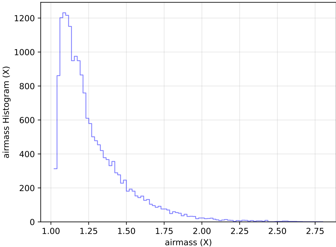
internal_u_expt38_nscale1.5v3.4_10yrs Yr 1 u band: airmass Histogram
