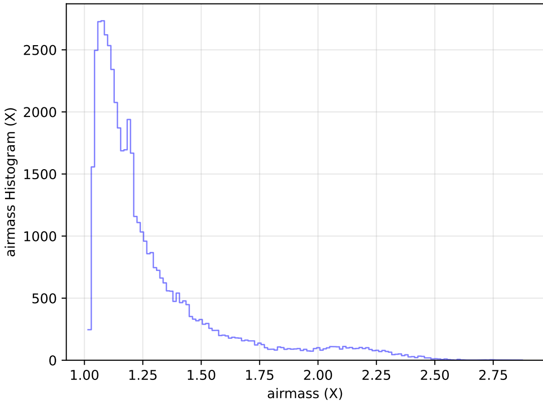
internal_u_expt38_nscale1.5v3.4_10yrs Yr 1 r band: airmass Histogram
