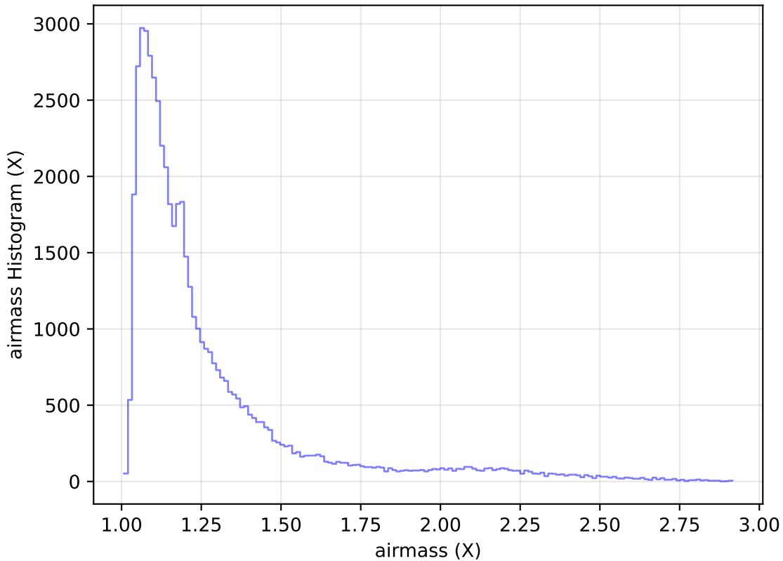
internal_u_expt38_nscale1.5v3.4_10yrs Yr 1 i band: airmass Histogram
