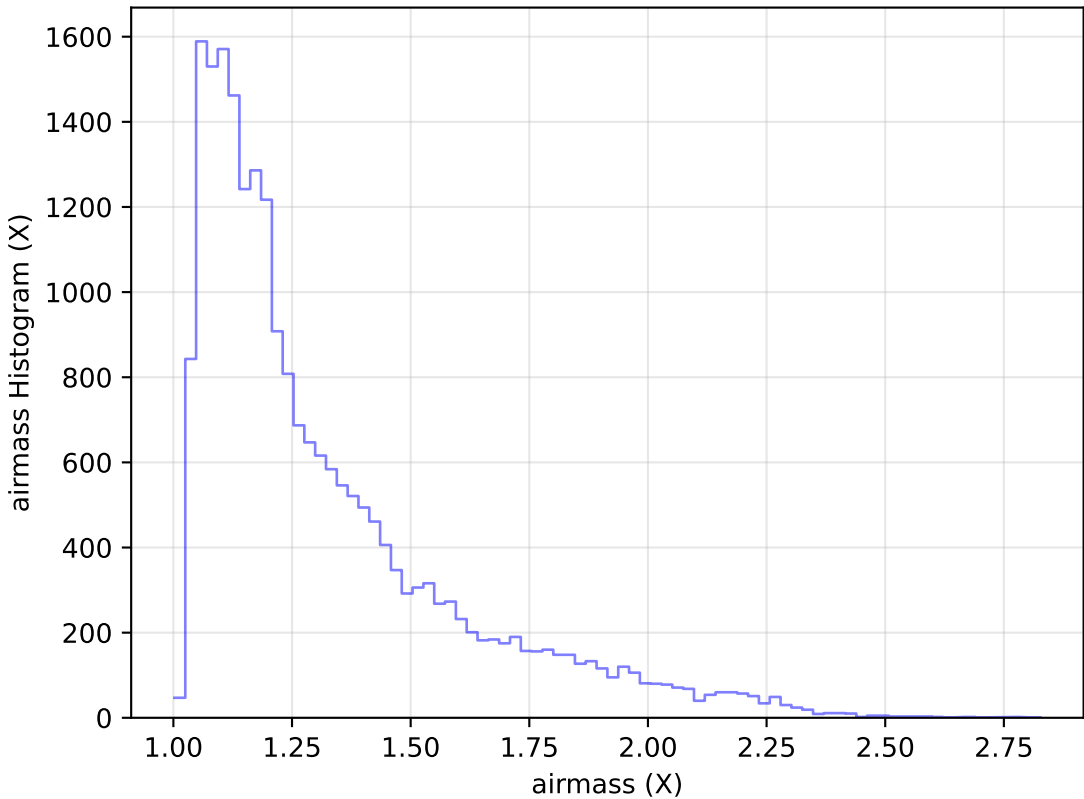
internal_u_expt38_nscale1.5v3.4_10yrs Yr 1 g band: airmass Histogram
