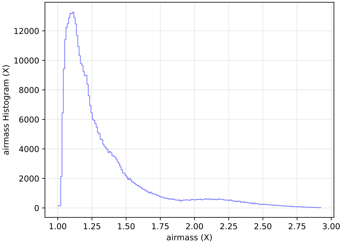
internal_u_expt38_nscale1.5v3.4_10yrs WFD z band: airmass Histogram
