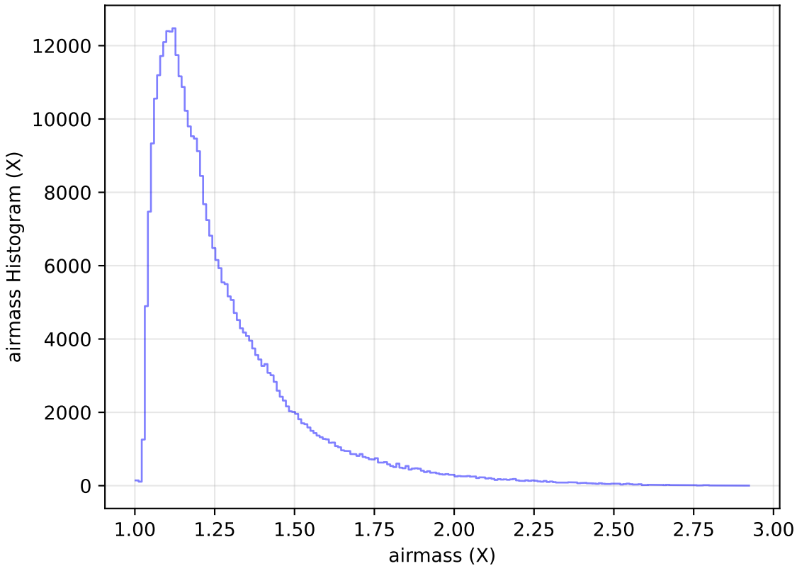
internal_u_expt38_nscale1.5v3.4_10yrs WFD y band: airmass Histogram
