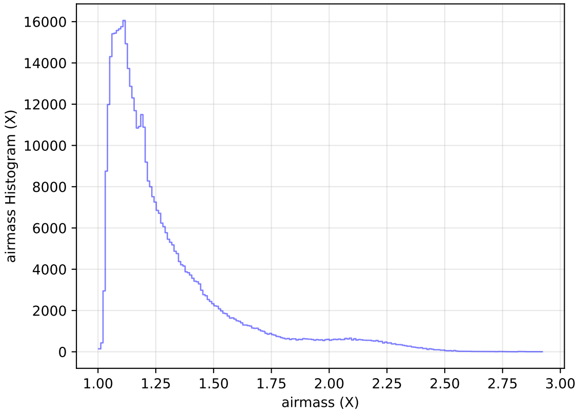
internal_u_expt38_nscale1.5v3.4_10yrs WFD r band: airmass Histogram
