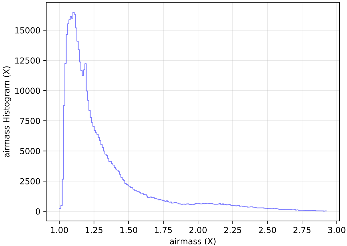
internal_u_expt38_nscale1.5v3.4_10yrs WFD i band: airmass Histogram
