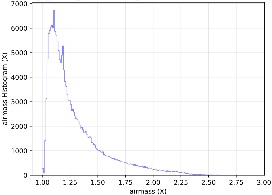
internal_u_expt38_nscale1.5v3.4_10yrs WFD g band: airmass Histogram
