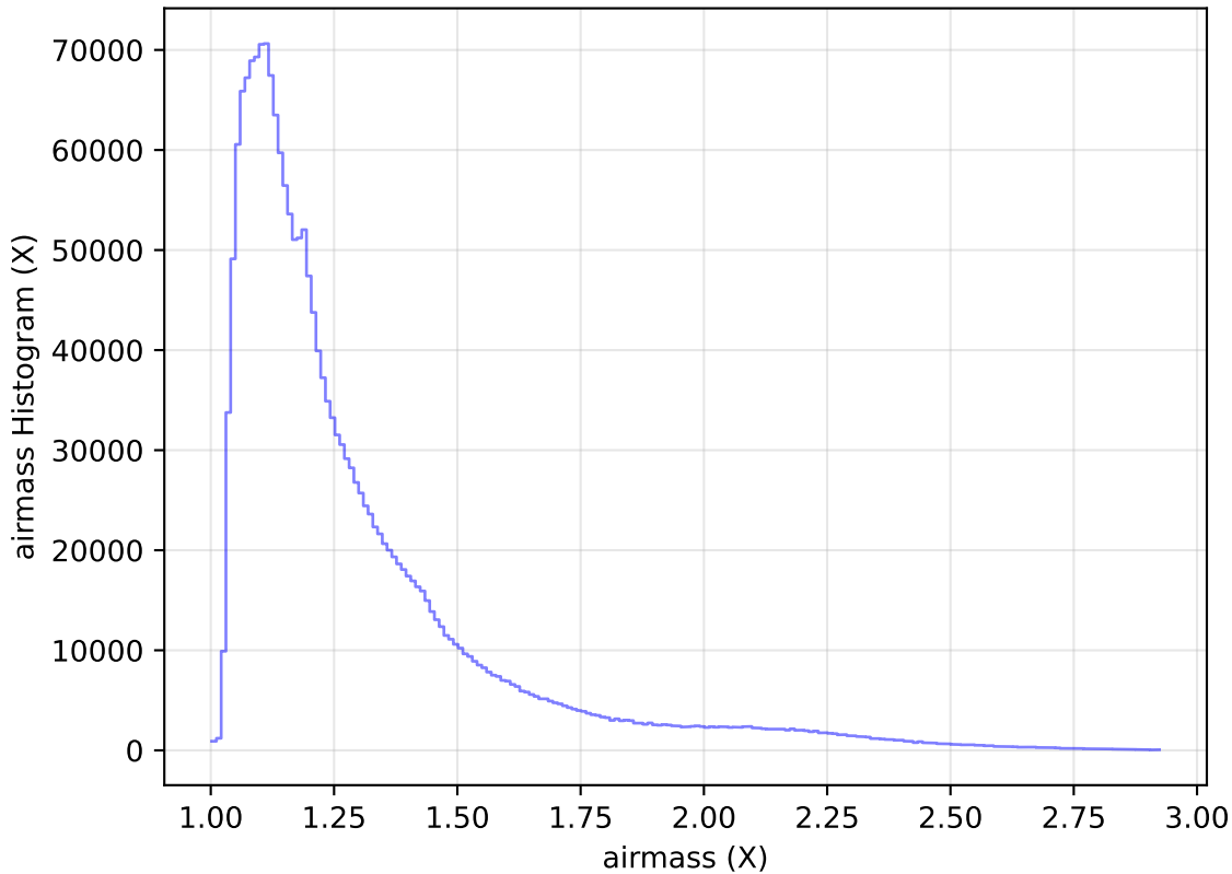
internal_u_expt38_nscale1.5v3.4_10yrs WFD all bands: airmass Histogram
