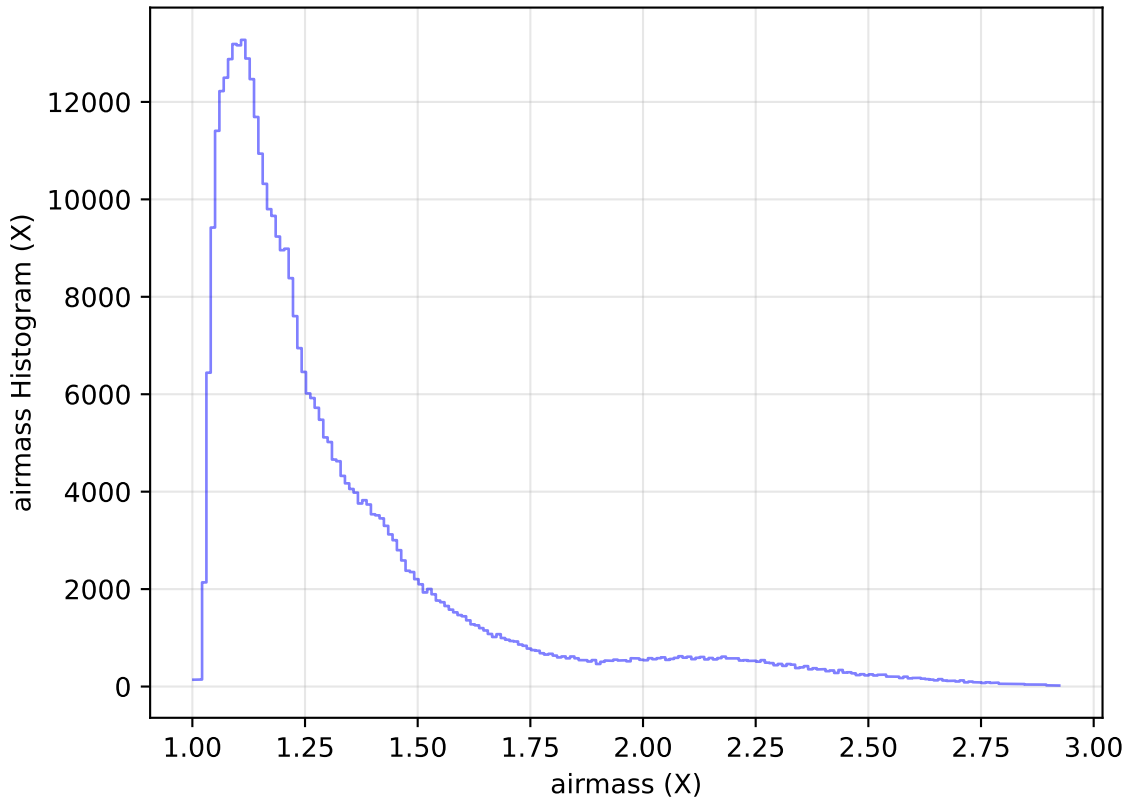
internal_u_expt38_nscale1.5v3.4_10yrs All sky z band: airmass Histogram
