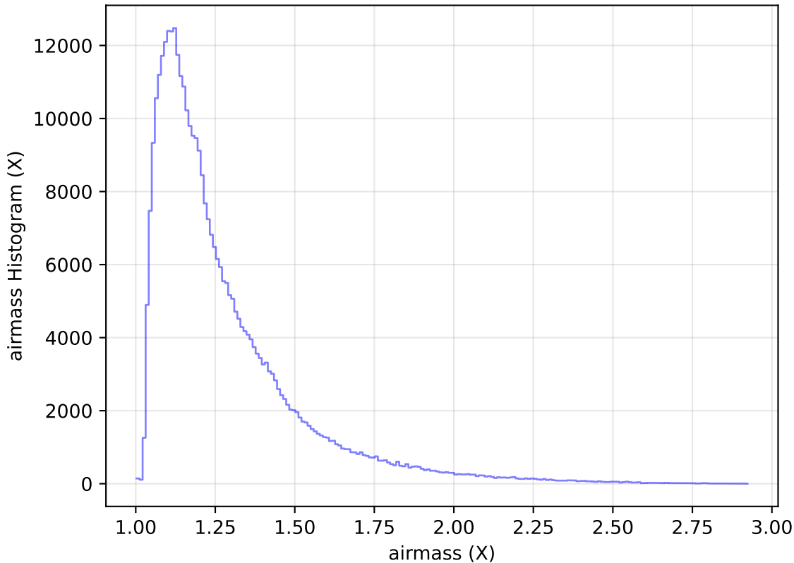
internal_u_expt38_nscale1.5v3.4_10yrs All sky y band: airmass Histogram
