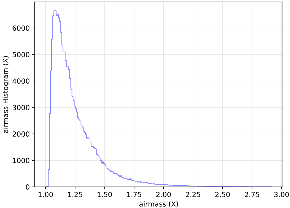
internal_u_expt38_nscale1.5v3.4_10yrs All sky u band: airmass Histogram
