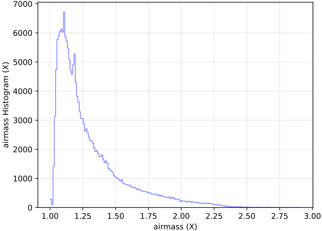
internal_u_expt38_nscale1.5v3.4_10yrs All sky g band: airmass Histogram
