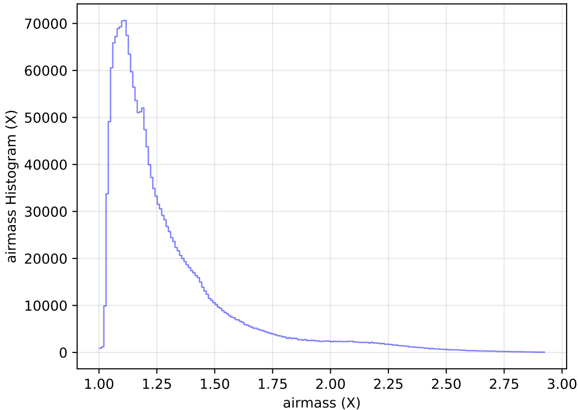
internal_u_expt38_nscale1.5v3.4_10yrs All sky all bands: airmass Histogram
