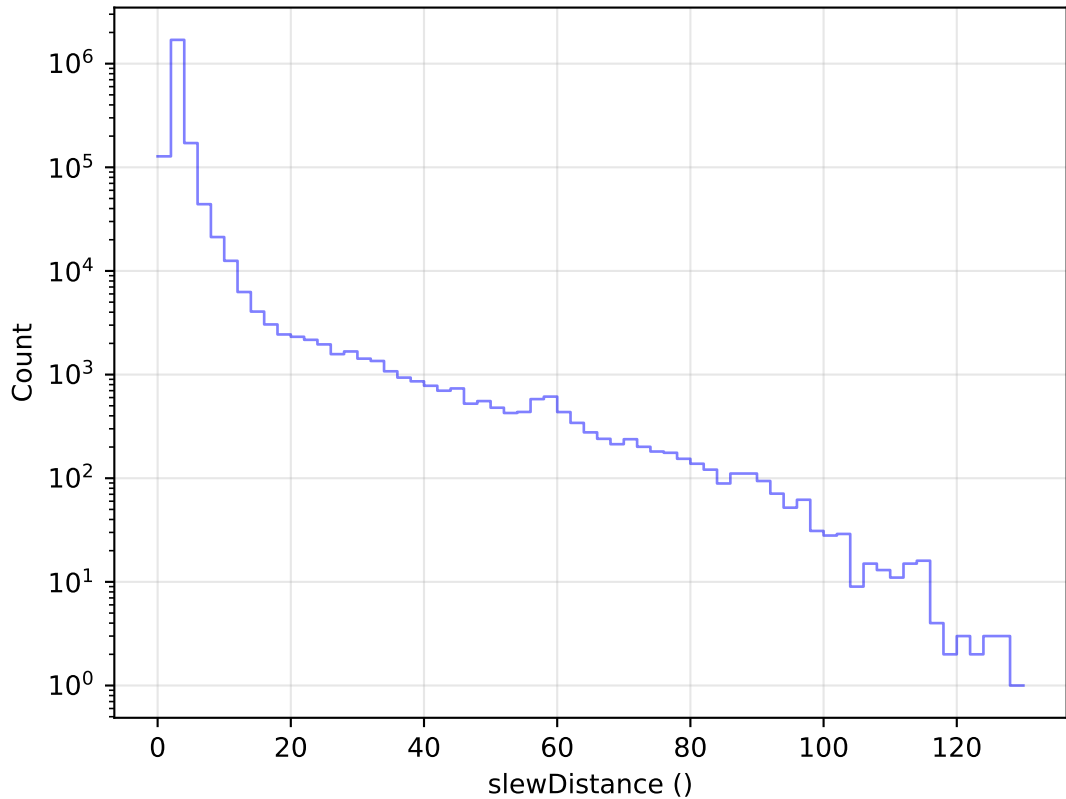
internal_u_expt38_nscale1.5v3.4_10yrs All visits: Slew Distance Histogram
