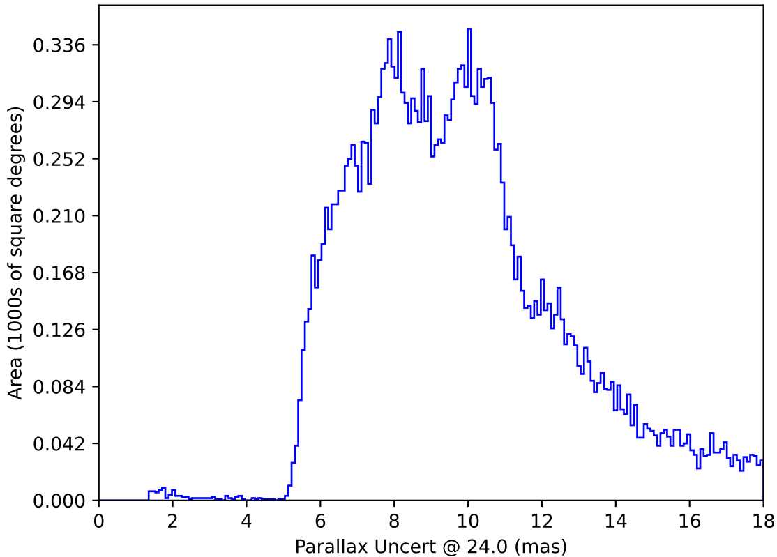
internal_u_expt38_nscale1.5v3.4_10yrs All sky: Parallax Uncert @ 24.0
