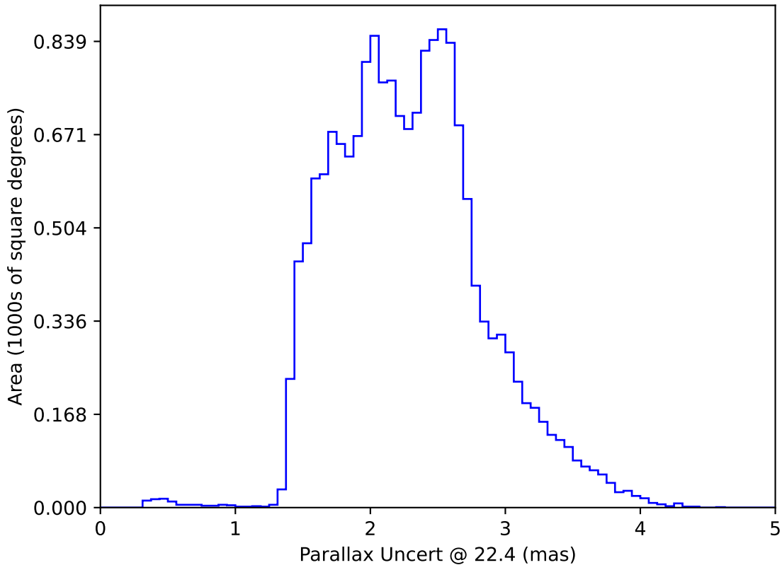
internal_u_expt38_nscale1.5v3.4_10yrs WFD: Parallax Uncert @ 22.4
