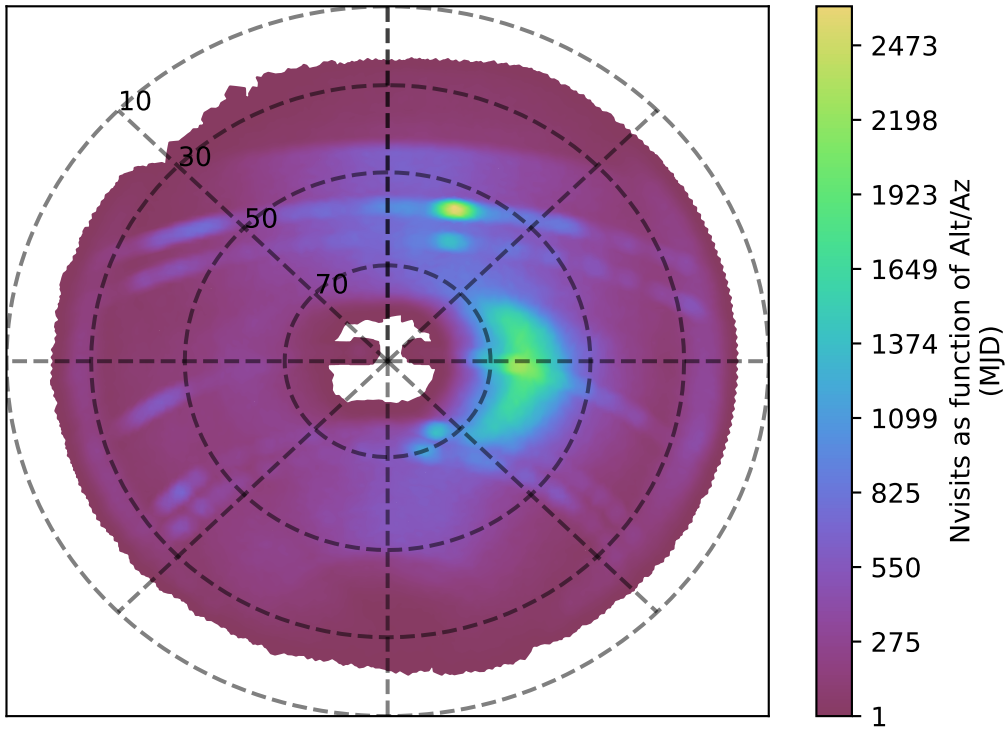
internal_u_expt38_nscale1.5v3.4_10yrs z band: Nvisits as function of Alt/Az
