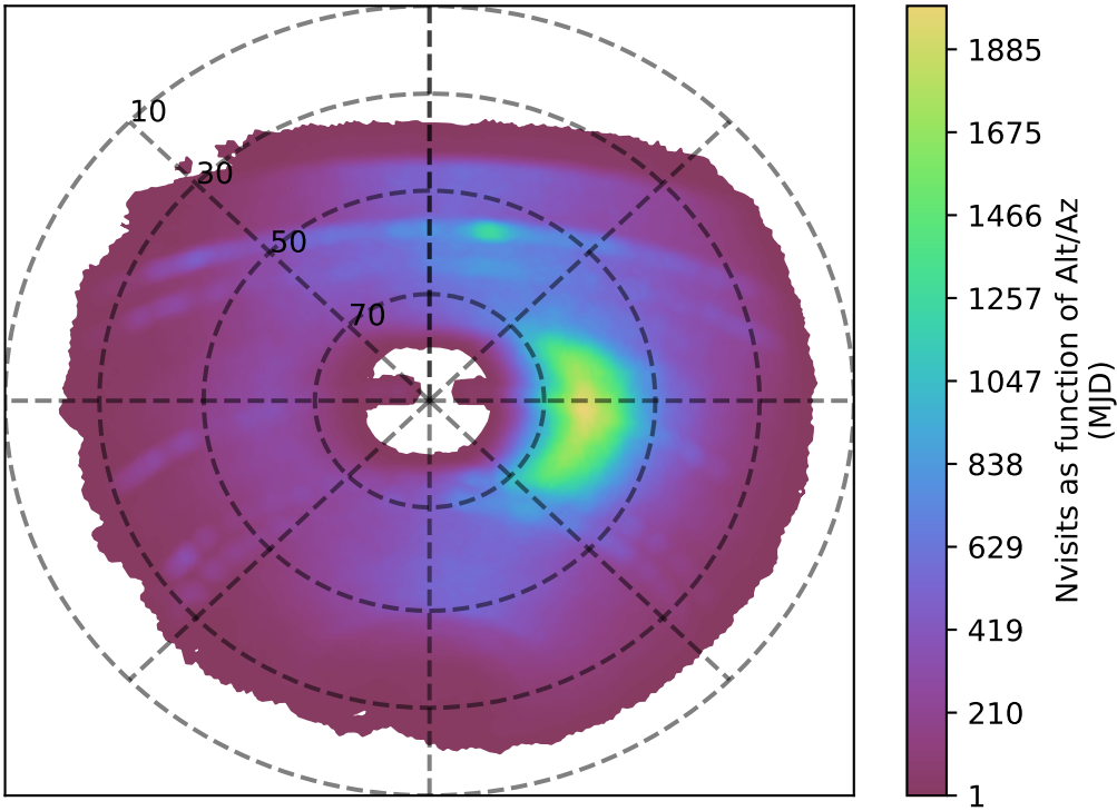
internal_u_expt38_nscale1.5v3.4_10yrs y band: Nvisits as function of Alt/Az
