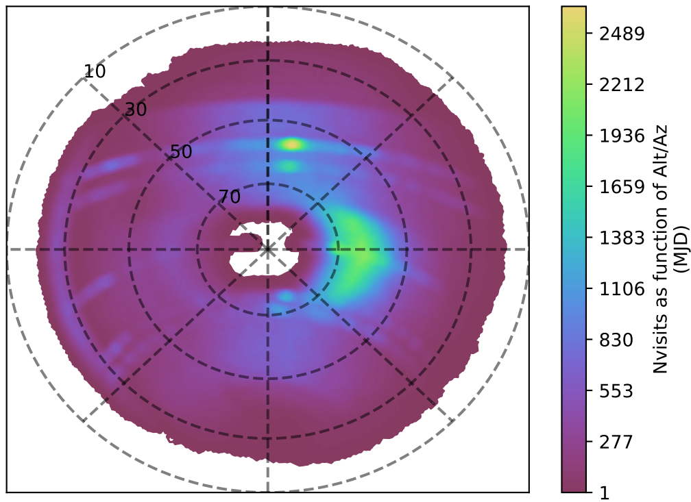
internal_u_expt38_nscale1.5v3.4_10yrs r band: Nvisits as function of Alt/Az
