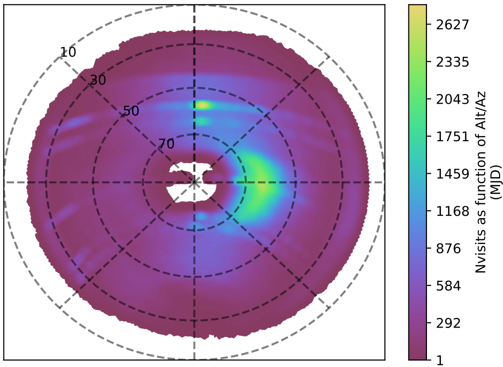
internal_u_expt38_nscale1.5v3.4_10yrs i band: Nvisits as function of Alt/Az
