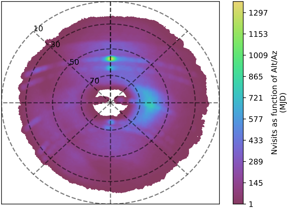
internal_u_expt38_nscale1.5v3.4_10yrs g band: Nvisits as function of Alt/Az
