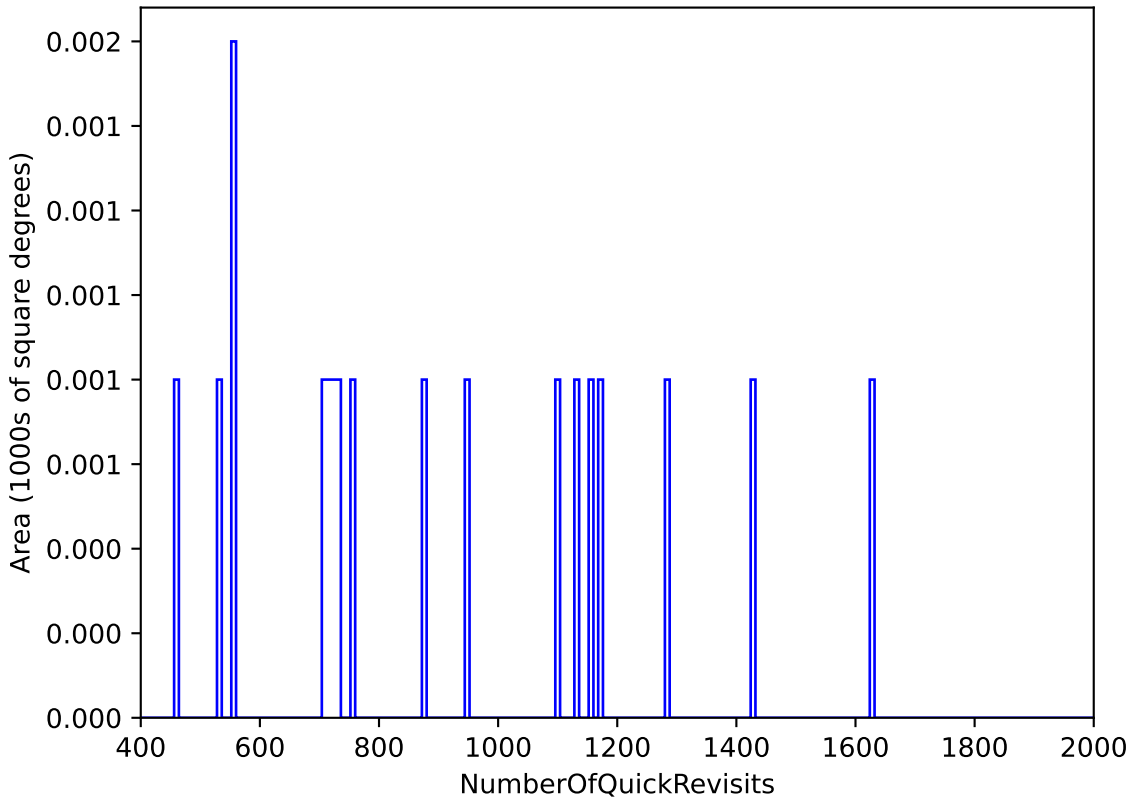
internal_u_expt38_nscale1.5v3.4_10yrs WFD: NumberOfQuickRevisits
