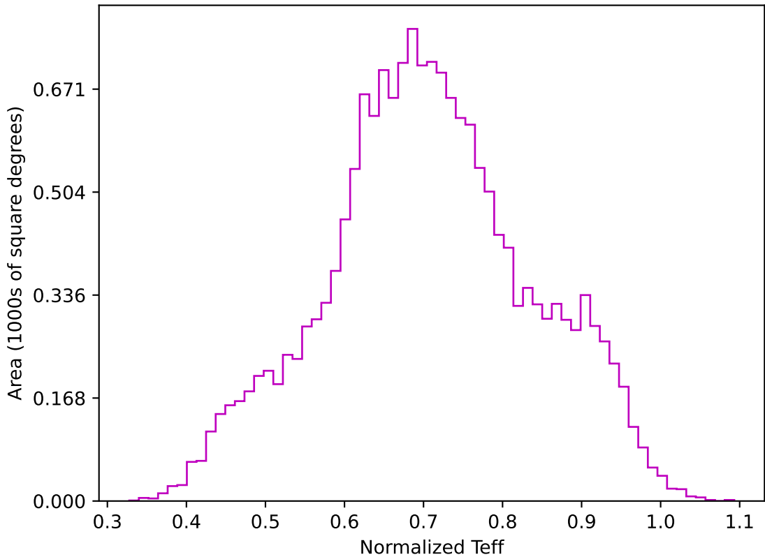
internal_u_expt38_nscale1.5v3.4_10yrs WFD z band: Normalized Teff
