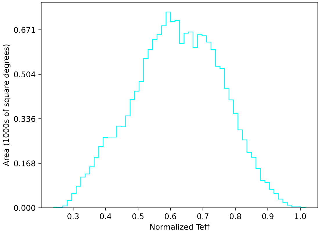
internal_u_expt38_nscale1.5v3.4_10yrs WFD u band: Normalized Teff
