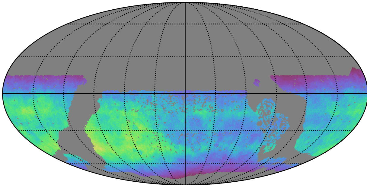
internal_u_expt38_nscale1.5v3.4_10yrs WFD i band: Normalized Teff
