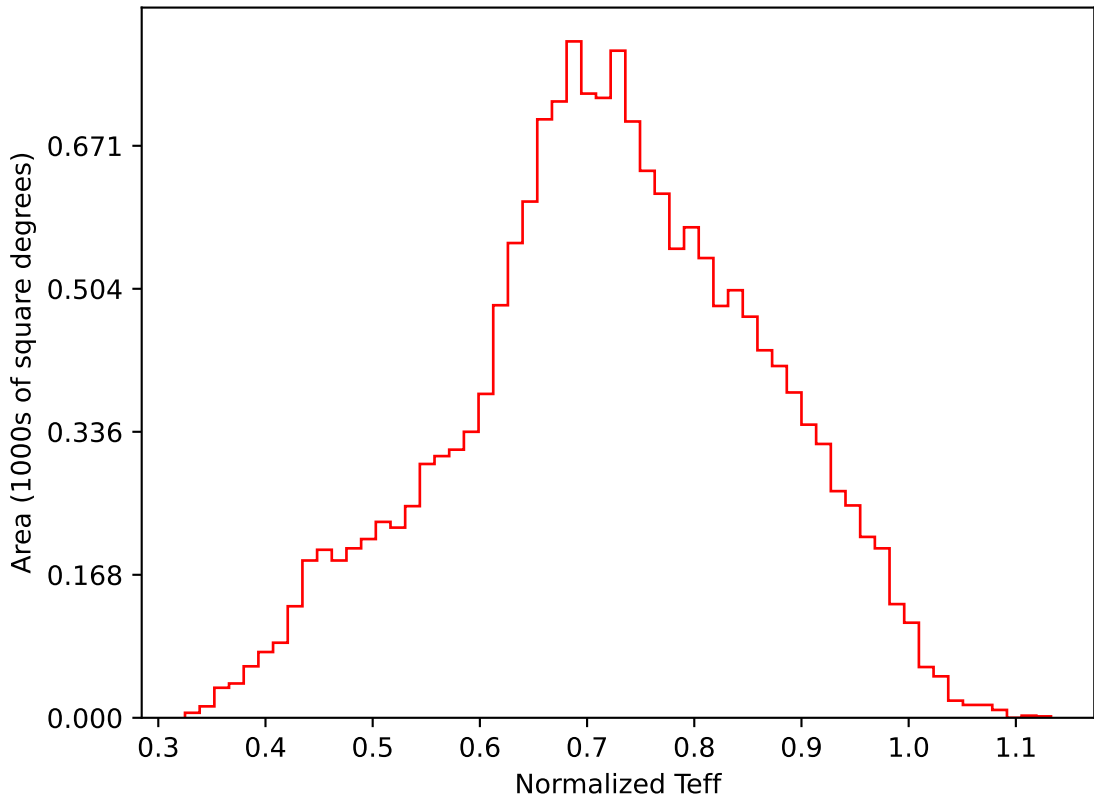
internal_u_expt38_nscale1.5v3.4_10yrs WFD i band: Normalized Teff
