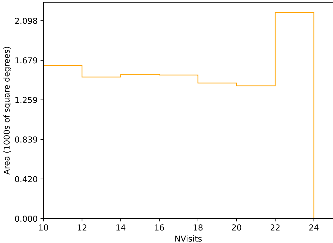
internal_u_expt38_nscale1.5v3.4_10yrs Yr 3-4 r band: NVisits
