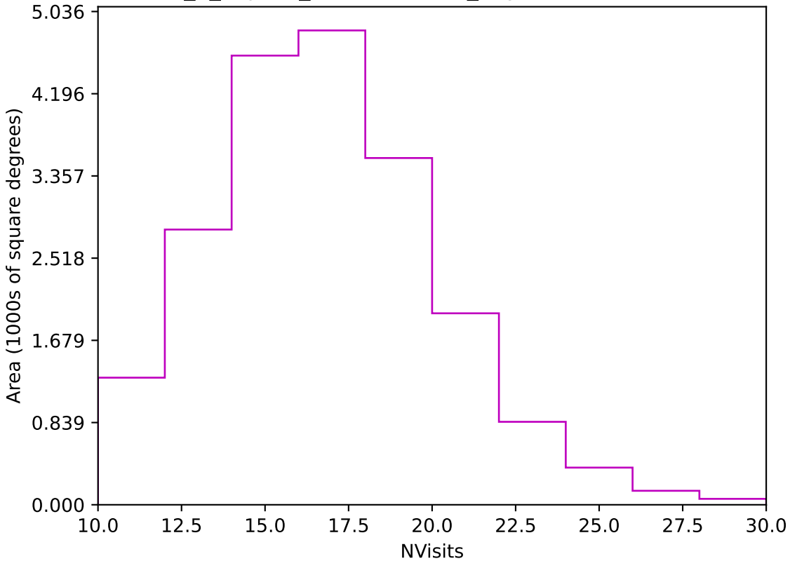
internal_u_expt38_nscale1.5v3.4_10yrs Yr 1 z band: NVisits
