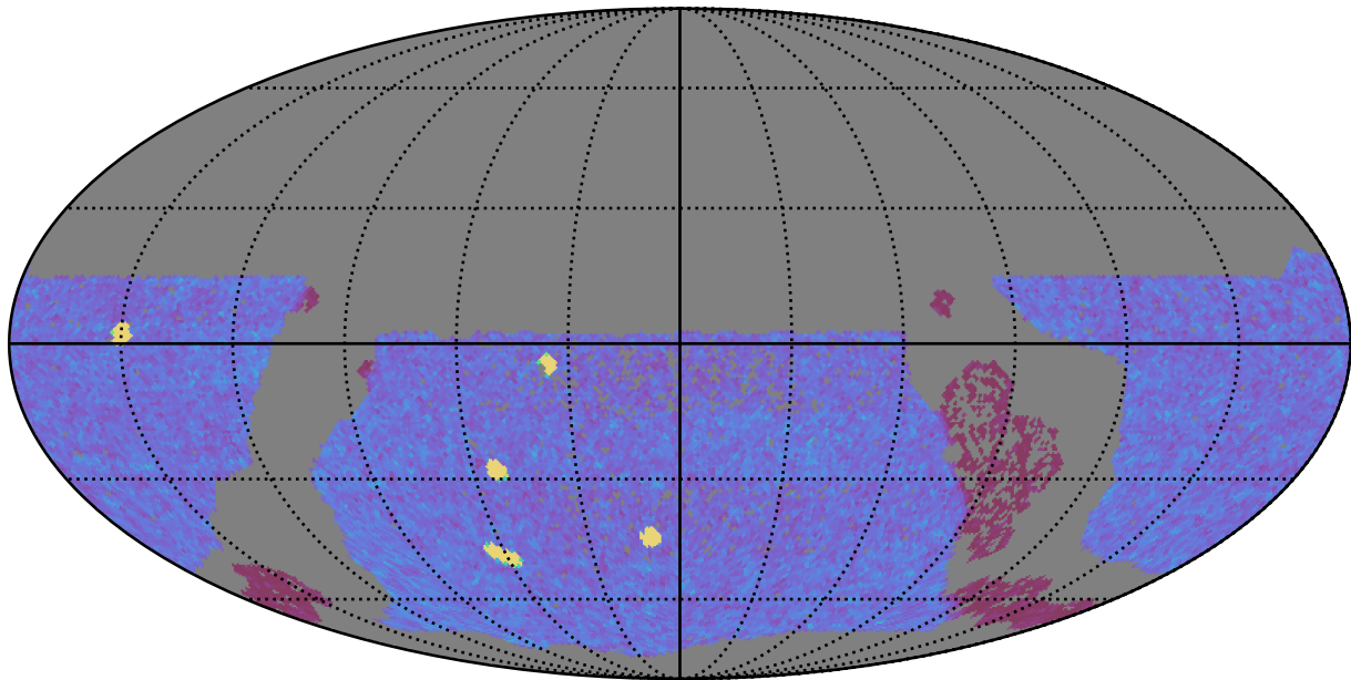
internal_u_expt38_nscale1.5v3.4_10yrs WFD y band: NVisits
