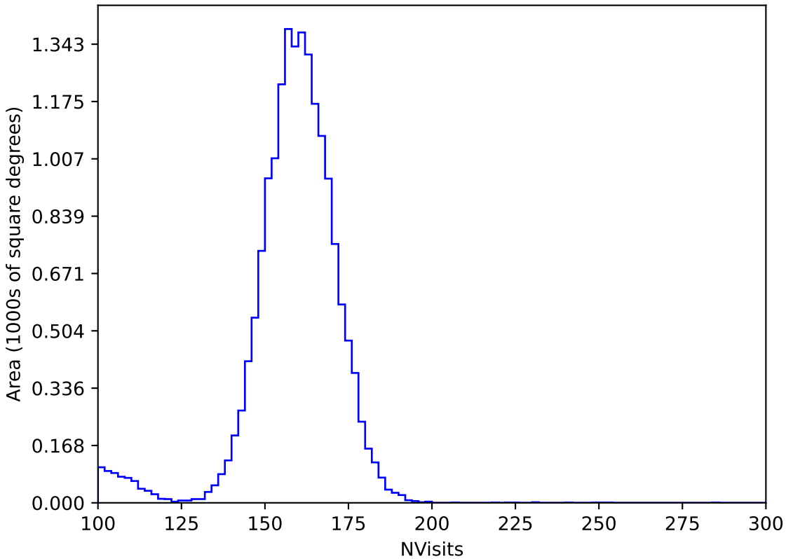
internal_u_expt38_nscale1.5v3.4_10yrs WFD y band: NVisits
