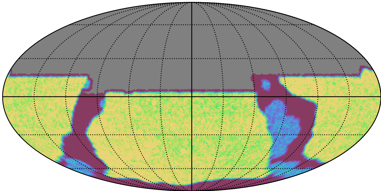
internal_u_expt38_nscale1.5v3.4_10yrs All sky u band: NVisits
